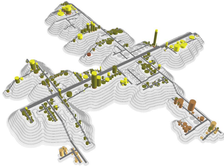
FIGURE 2.6: Representing Development History in Software Cities [47]
